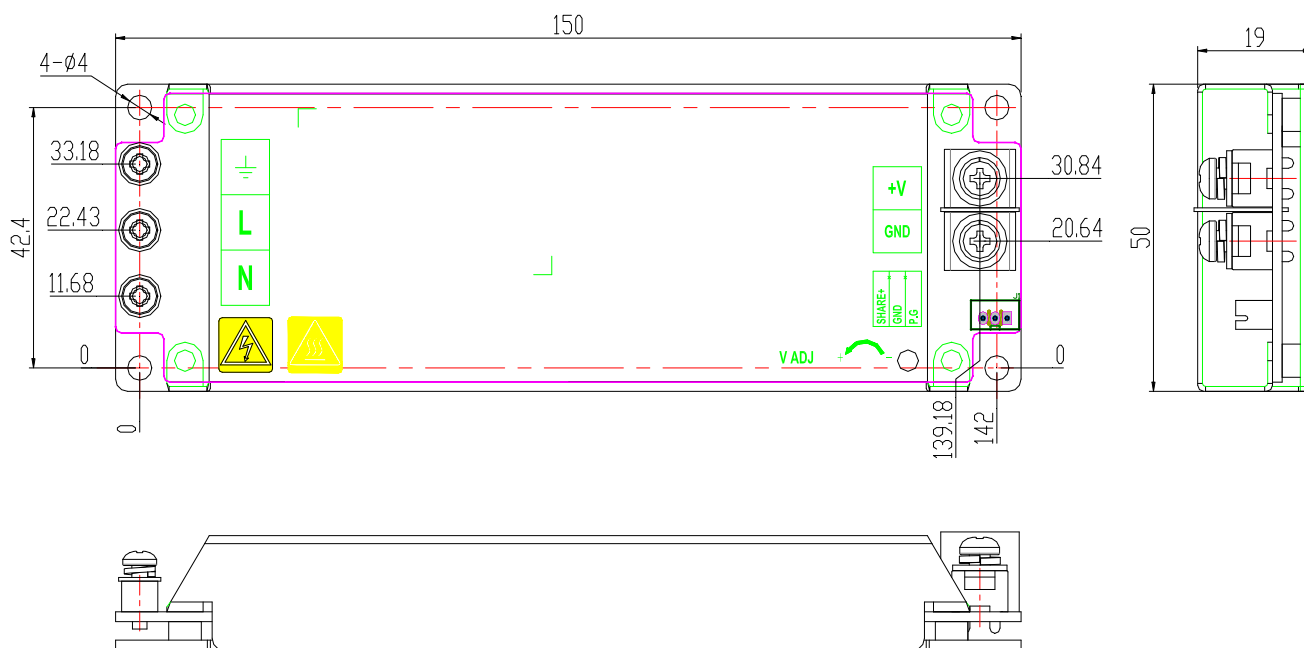
Dimension and mounting hole -- terminal coordinate drawing
